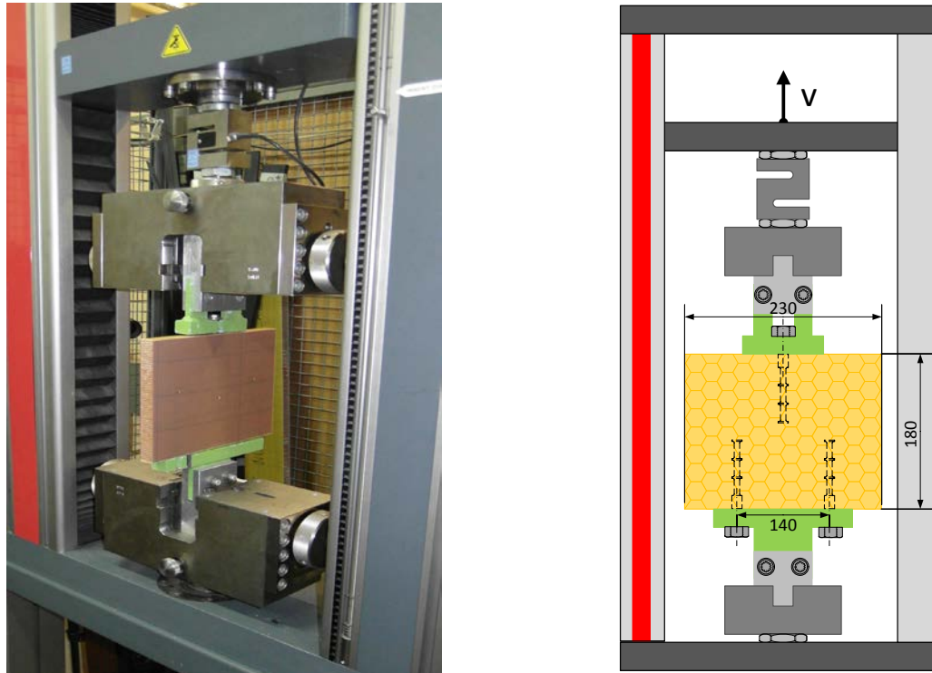
Figure 4 Experimental setup
