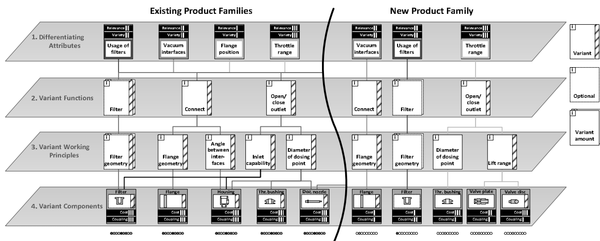
Figure 5. VAM detail of the existing product families (left) and the new product family (right)
