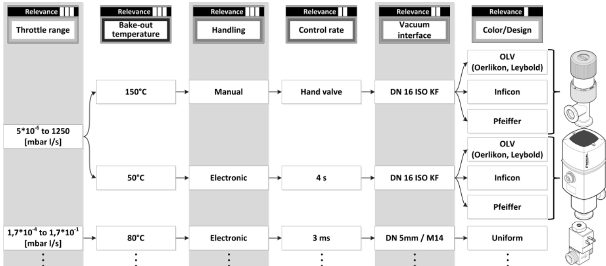
Figure 2. Tree of variety of the existing product families
