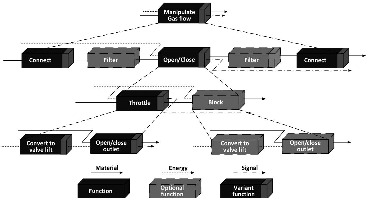
Figure 3. Hierarchical function structure of the existing product families
