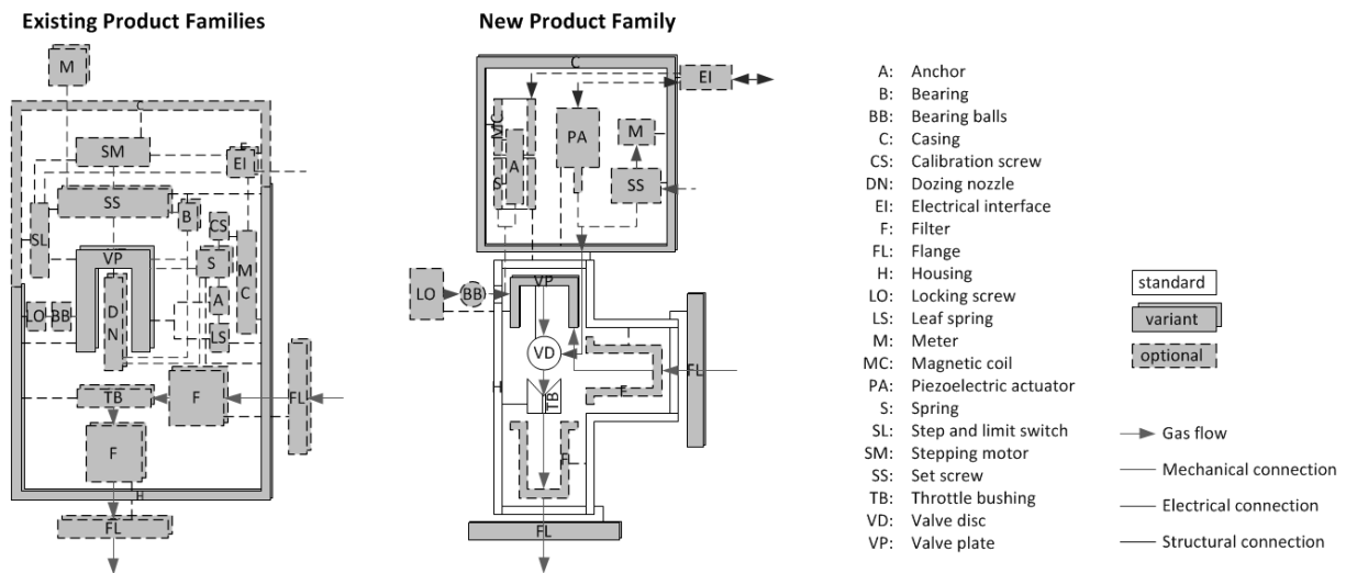
Figure 4. MIGs of the existing valves (left) and the new product family (right)
