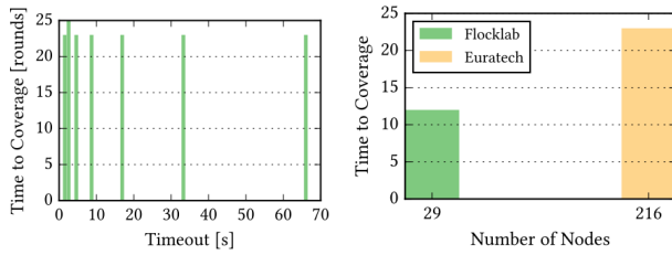
(a) Election timeout does not affect convergence time. The Euratech network converges within 23 rounds = 41 seconds on average. (b) Leader election on a sparse and a dense testbed; respectively, Flocklab and Euratech.
